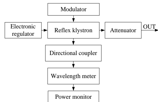
Fig. 3: Microwave signal generator block diagram
