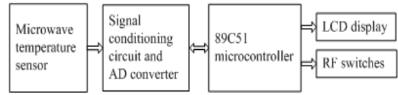
Fig. 1: Microwave temperature measurement block diagram
