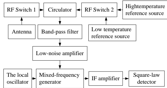
Fig. 2: The block diagram of the microwave temperature sensor
