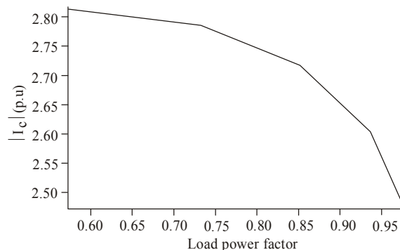
Fig. 6: The effect of power factor variation on the injecting current of the D-STATCOM under 25% voltage sag
