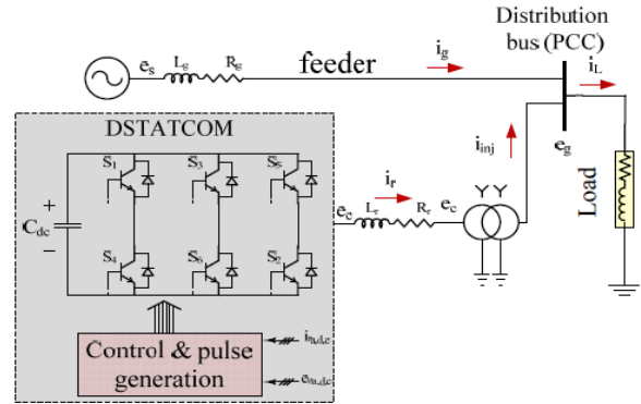
Fig. 1: The D-STATCOM structure (Hingorani et al. , 1999)
