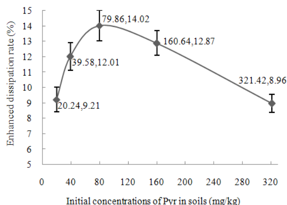
Fig. 3: Enhanced dissipation rates of pyrene in soils at different pollution levels by Tween 80
