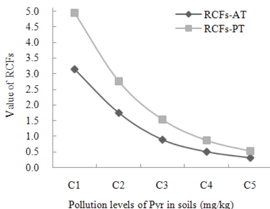
Fig. 4: RCFs of pyrene as a function of PAHs concentrations in soils (RCFs-PT and RCFs-AT denoted root concentration factors in soils at the presence and absence of Tween 80, respectively)
