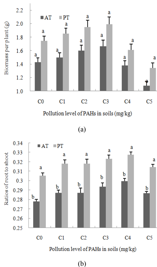
Fig. 1: Biomass and ratios of root to shoot of plants grown in treated soils; (PT and AT denoted the Pyr-spiked soils at the presence and absence of 4% Tween 80, respectively); (a): Biomass; (b): Ratios of root to shoot
