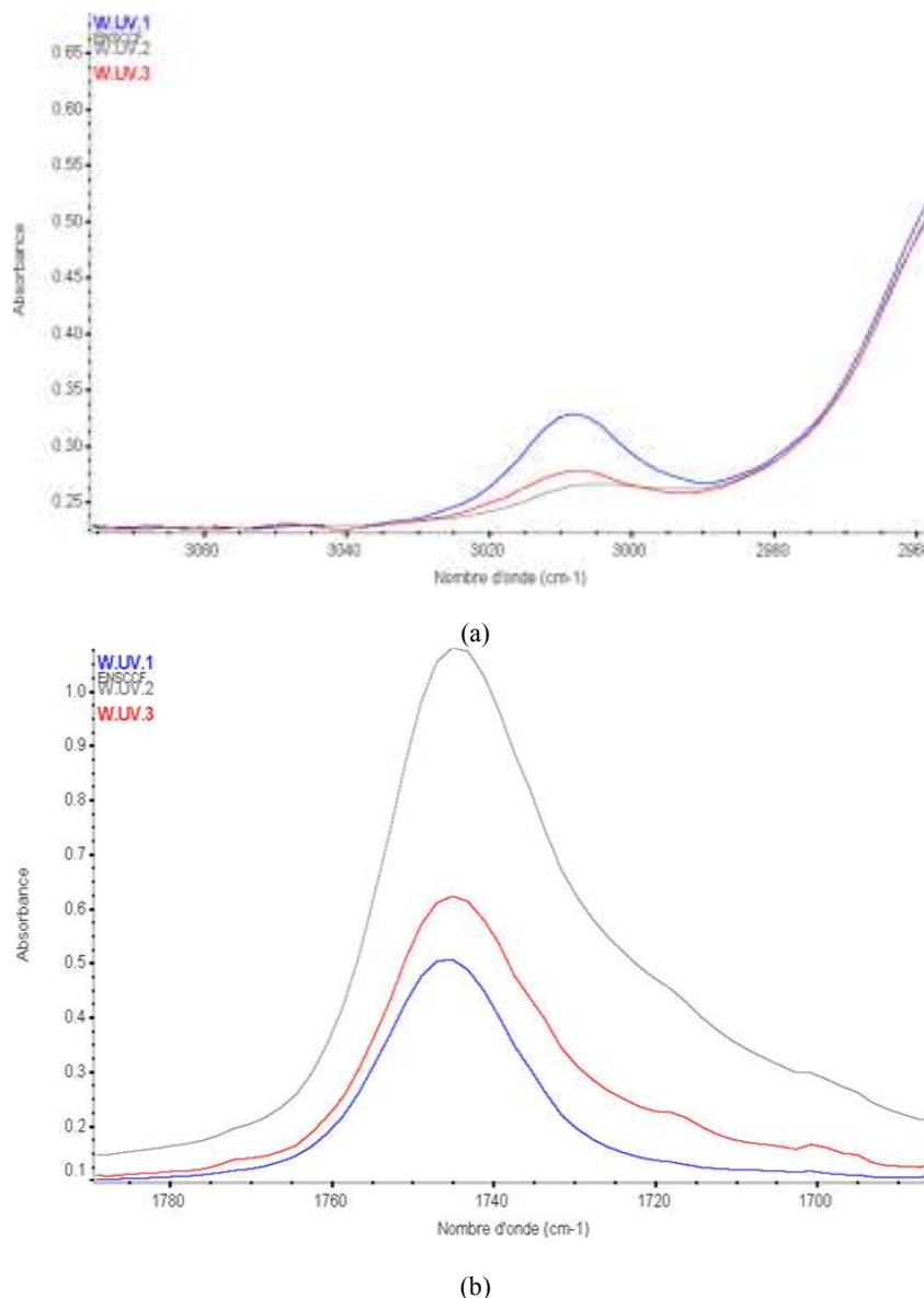
Fig. 2: Evolution of the grouping (a) and of esters (b) of FA during the action of UV (Blue: 60 min; Grey: 240 min; Red: 1440 min)
