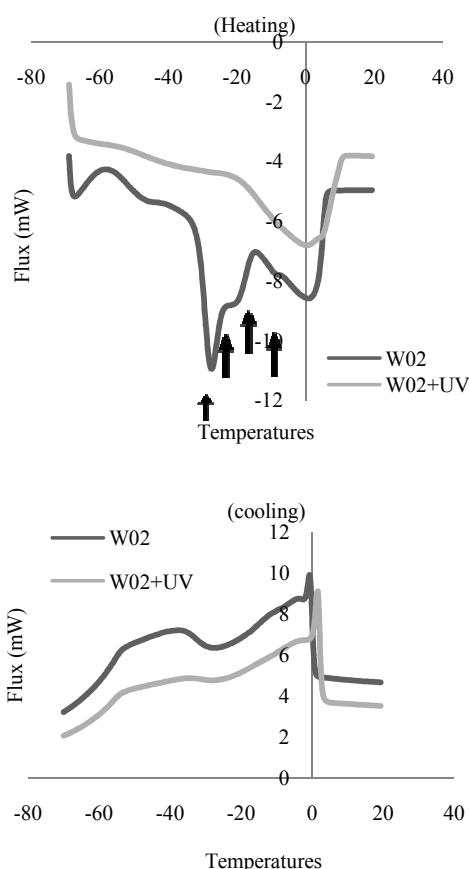
Fig. 3: Compared behavior compared between W02 sample having undergone UV action and W02 sample
