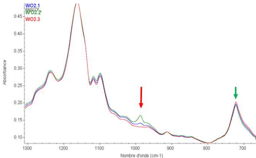
Fig. 6: Screen photo showing behavior variations of pumpkin seed oil matrix. (Blue: 60 min; green: 240 min; red: 1440 min)
