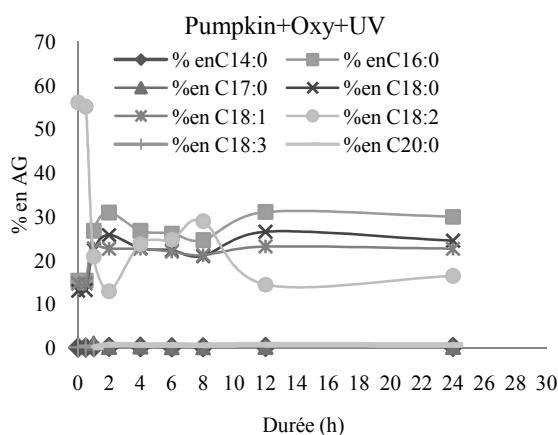
Fig. 8: FA contents behavior during accumulated action
