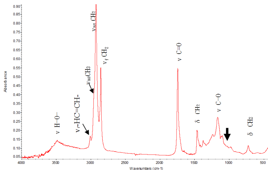
Fig. 1: W02 + UV. After 1440 min followed by a solvent evaporation
