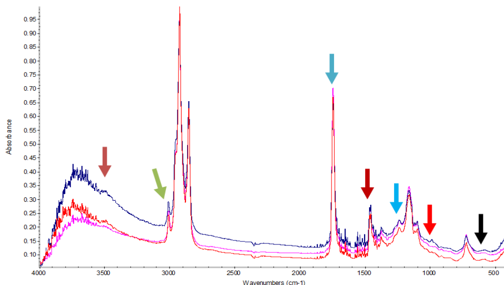
Fig. 4: Comparison of oxygen action on pumpkin seed oil; Red: 60 min; Blue: 240 min; Purple: 1440 min
