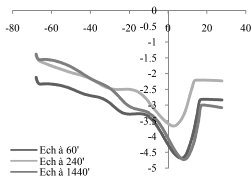
Fig. 7: Behavior of different AG families during air dioxygen action followed by DSC
