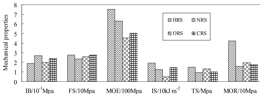
Fig. 3: Effect of treatments on mechanical properties of composites
