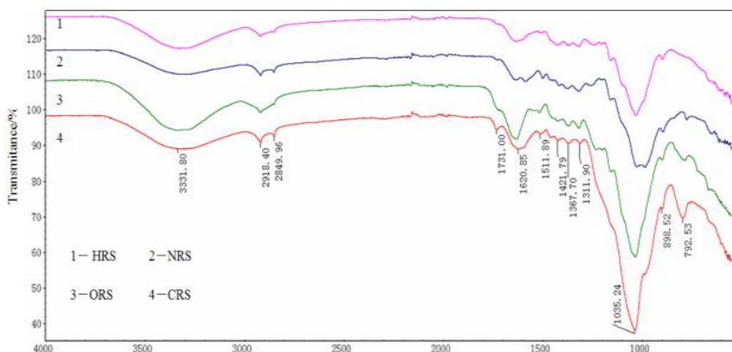
Fig. 1: FTIR of rice straw
