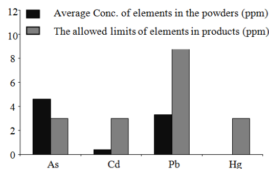
Fig. 4: The averages concentration of metals in the powder products compared to allowed limits
