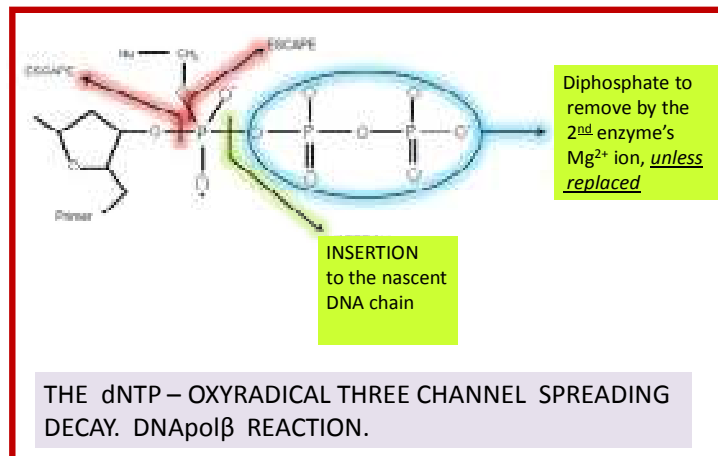
Fig. 5: The dNTP-oxyradical three channel spreading decay. DNAPol \beta reaction
