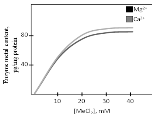
Fig. 7: An impact of the metal incubation mixture concentration on exogenous ions incorporation into the DNAPolβ structure (20 mM MeCl 2 /15 mM Tris-HCl (pH 8.0)/1.5 mM EDTA/+37°C/2 h)
