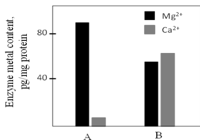
Fig. 6: The highest-reachable levels of substitution of endogenous Mg 2+ with calcium in purified HL60 DNAPolβ (20 mM CaCl 2 /15 mM Tris-HCl (pH 8.0)/1.5 mM EDTA/+37°C/2 h); A-control (intact enzyme); B-experiment (Mg-Ca substitution)
