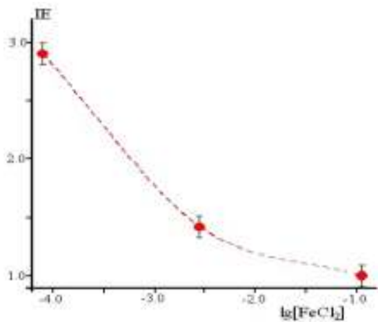
Fig. 4: Isotope Effect (IE) as a function of the \text{FeCl}_2 mM concentration, log scaled
