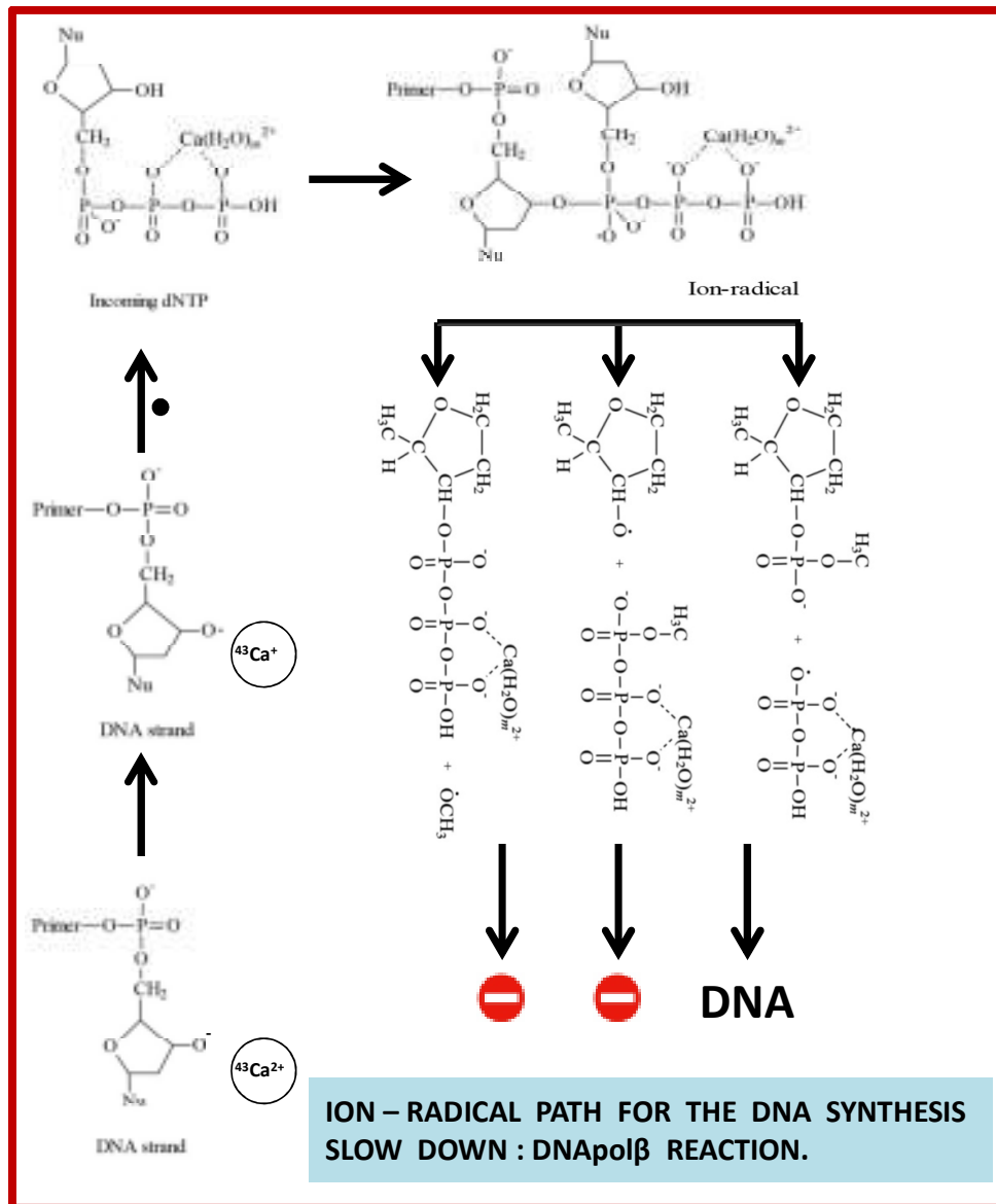
Fig. 1: ION-radical path for the DNA synthesis slow down: DNAPolβ reaction
