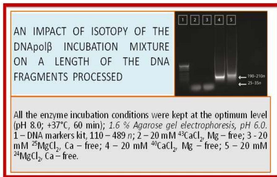
Fig. 2: An impact of isotope of the DNAPolβ incubation mixture on a length of the DNA fragments processed. Agarose gel electrophoresis; 1- DNA markers kit, 110 - 489 n; 2 - 20 mM 43 CaCl 2 , Mg - free; 3 - 20 mM 25 MgCl 2 , Ca - free; 4 - 20 mM 40 CaCl 2 , Mg - free; 5 - 20 mM 24 MgCl 2 , Ca - free; All the enzyme incubation conditions were kept at the optimum level (pH 8.0; +37°C, 60 min)
