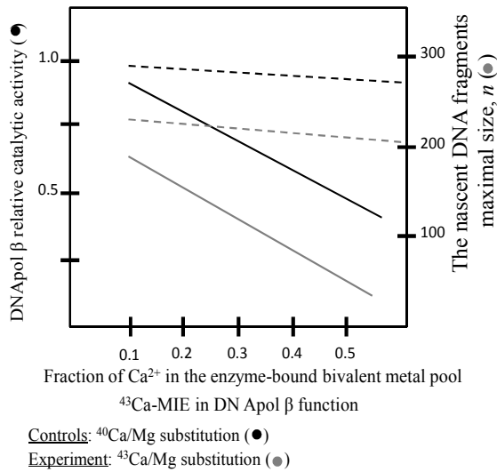
Fig. 3: Fraction of calcium in the enzyme-bound bivalent metal pool
