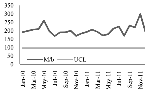
Fig. 1: Box M control chart
