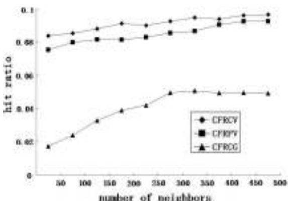
Fig. 2: hit ratio comparison
