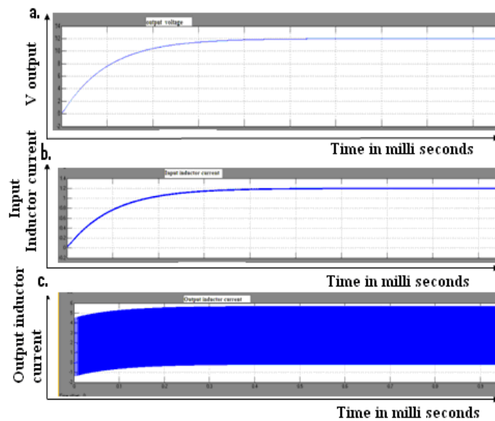
Fig. 8: (a) output voltage, (b) output current, (c) input current waveforms of SMC
