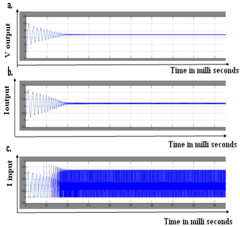
Fig. 6: (a) output voltage, (b) output current, (c) input current waveforms of PI controller
