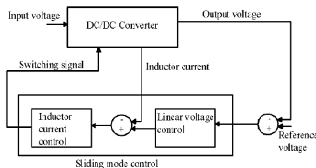
Fig. 2: Block diagram of sliding mode control of DC-DC converters
