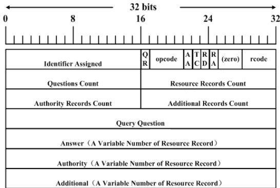
Fig. 5: The DNS data format
