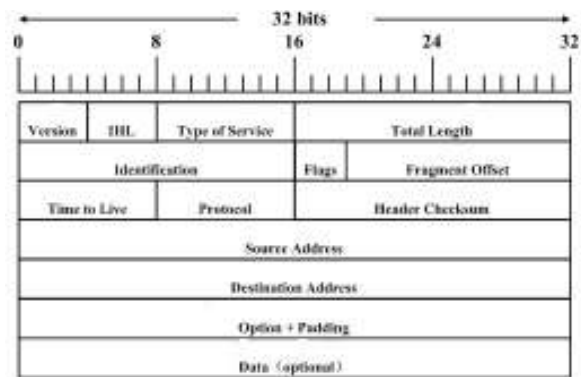
Fig. 2: The IP format
