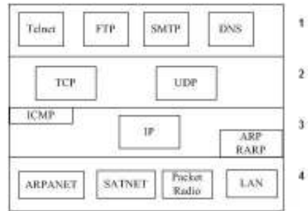
Fig. 1: TCP/IP architecture
