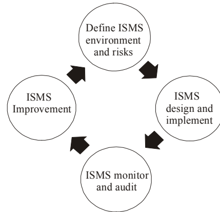
Fig. 1: ISMS Cycle
