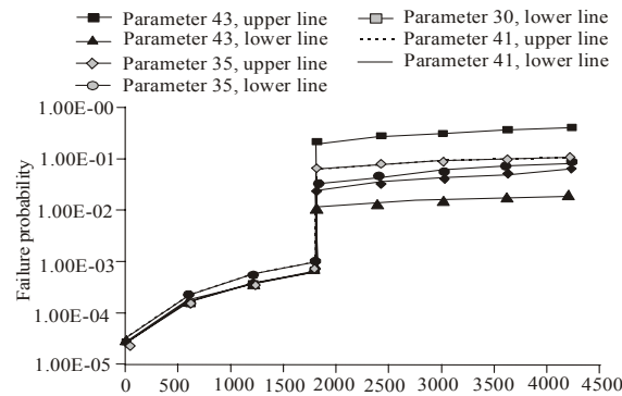
Fig. 9: Most sensitive parameter in phase 2
