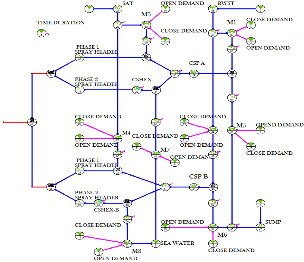
Fig. 6: GO-FLOW chart in case of two lines running simultaneously
