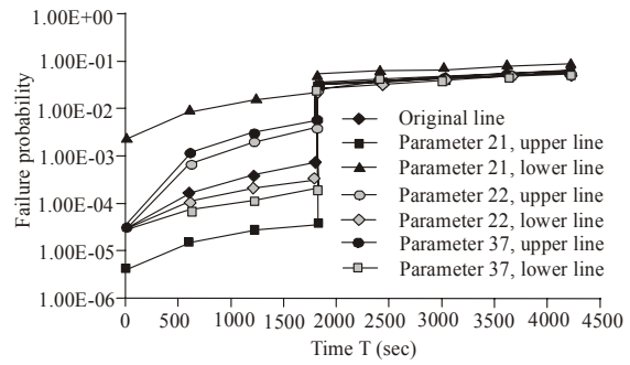
Fig. 8: Most sensitive parameter in phase 1
