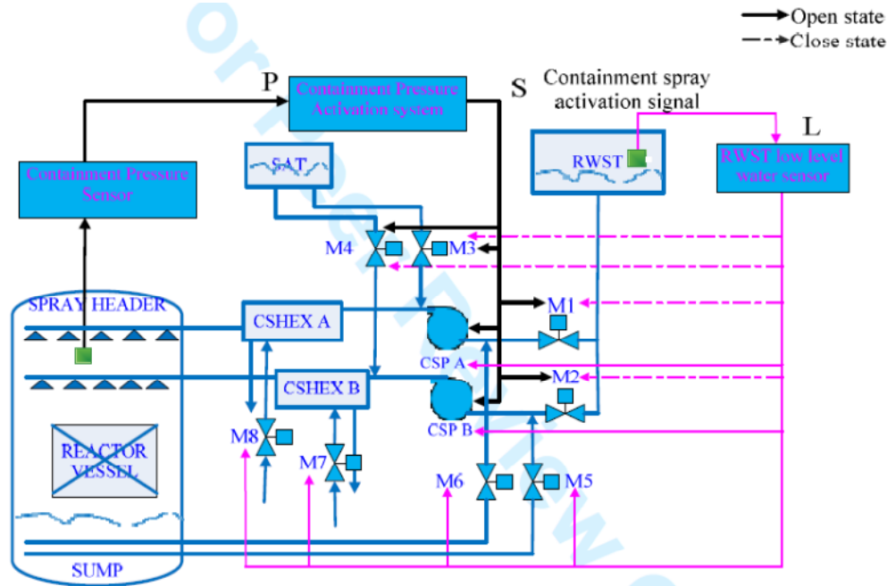
Fig. 5: Containment spray system in case of two lines running simultaneously
