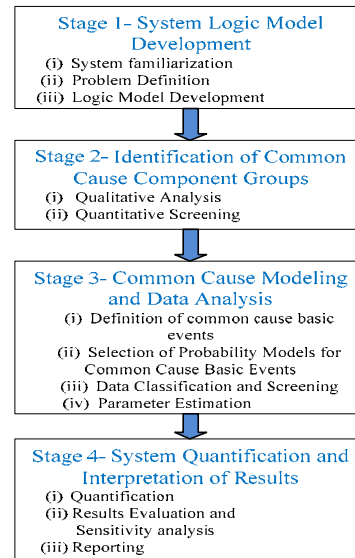
Fig. 3: Procedural framework for common cause failure analysis
