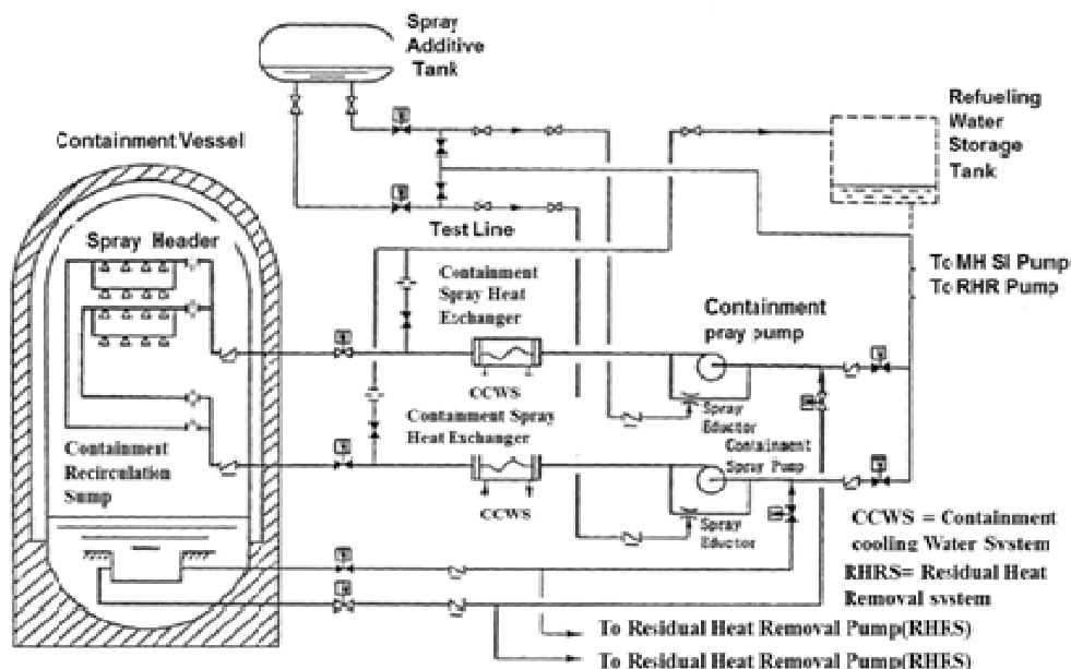
Fig. 4: Containment spray system of PWR plant
