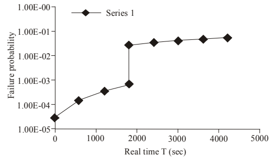
Fig. 7: Failure probability of containment spray system
