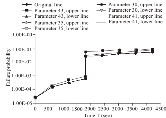
Fig. 10: Most sensitive parameter in phase 2
