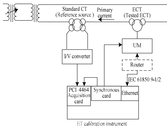
Fig. 1: Calibration system of digital output for ECT
