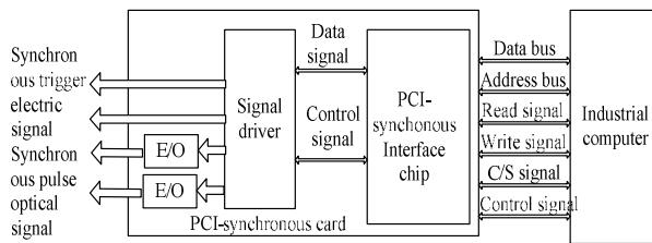
Fig. 3: Hardware diagram of data synchronization card
