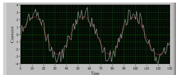
Fig. 5: Results of zero-phase filter test
