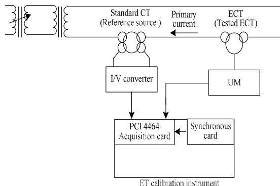
Fig. 2: Calibration system of analog output for ECT
