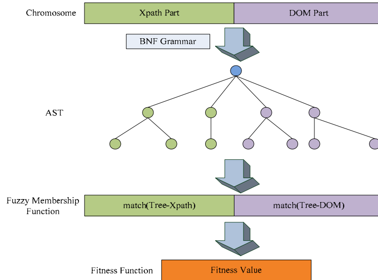
Fig. 5: Process of fitness value evaluation
