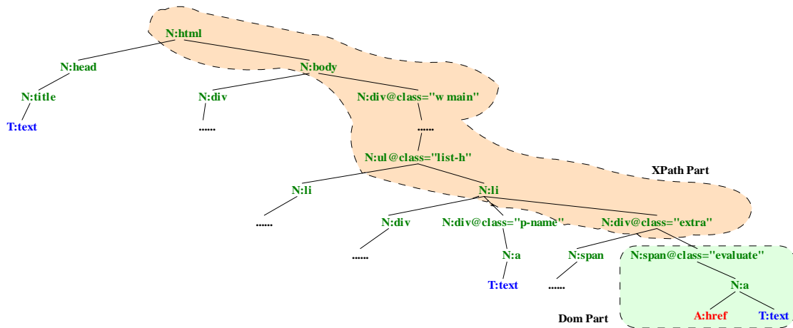
Fig. 4: DOM tree with Xpath and DOM parts
