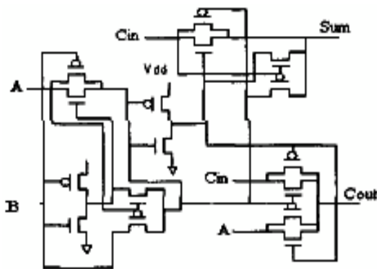
Fig. 3: The transmission function adder (TFA)
