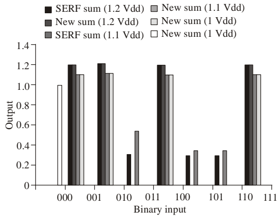
Fig. 7: Sum comparison
