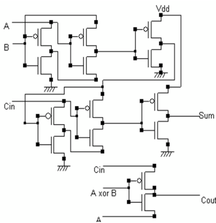
Fig. 6: New improved 14T Adder
