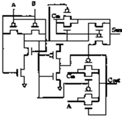
Fig. 5: The fourteen Transistor (14T) adder
