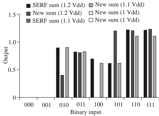
Fig. 8: Carry comparison
