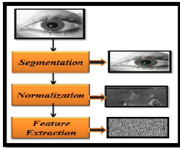
Fig. 3: Iris preprocessing
