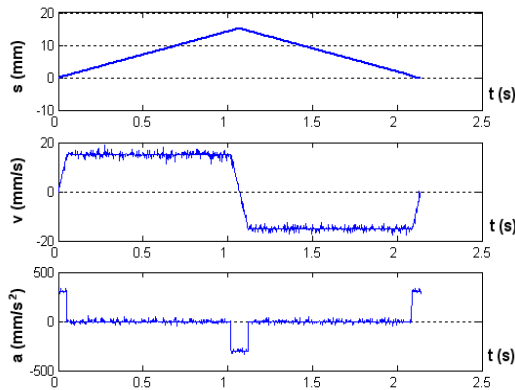
Fig. 8: Adopting the linear Acc/Dec approach
