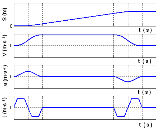
Fig. 5: The motion profile when S \geq S_3
