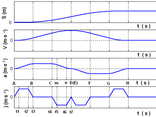
Fig. 2: The motion profile with displacement S_1
