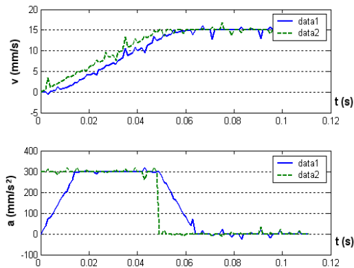
Fig. 9: Compare the two Acc/Dec approaches
