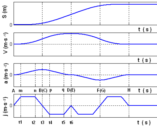
Fig. 4: The motion profile with displacement S_3
