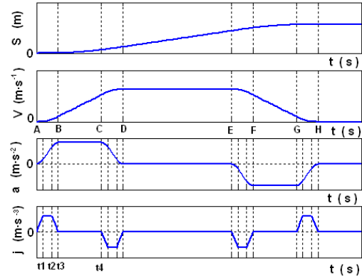
Fig. 1: Acc/Dec approach based on trapezoid-curve jerk
