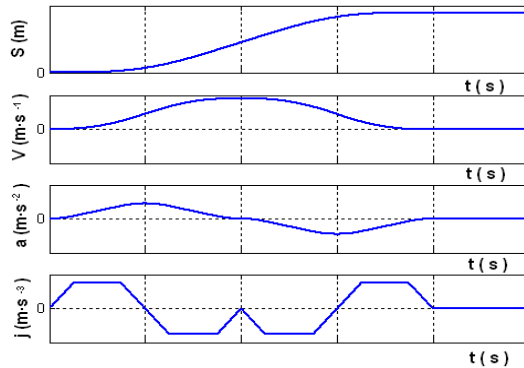
Fig. 3: The motion profile with displacement S_2
