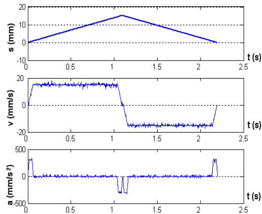
Fig. 7: Adopting the developed Acc/Dec approach
