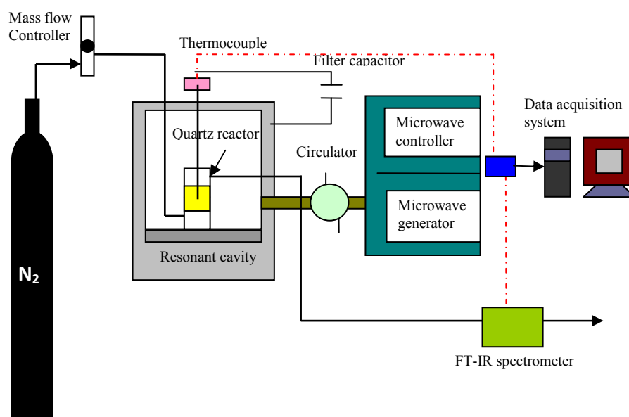
Fig. 1: Schematic diagram of microwave heating system
