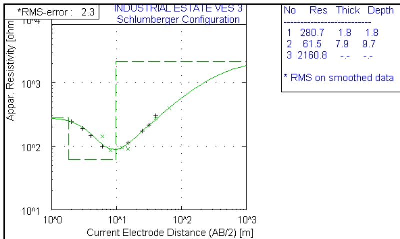
(c) The modeled curve for VES 3
