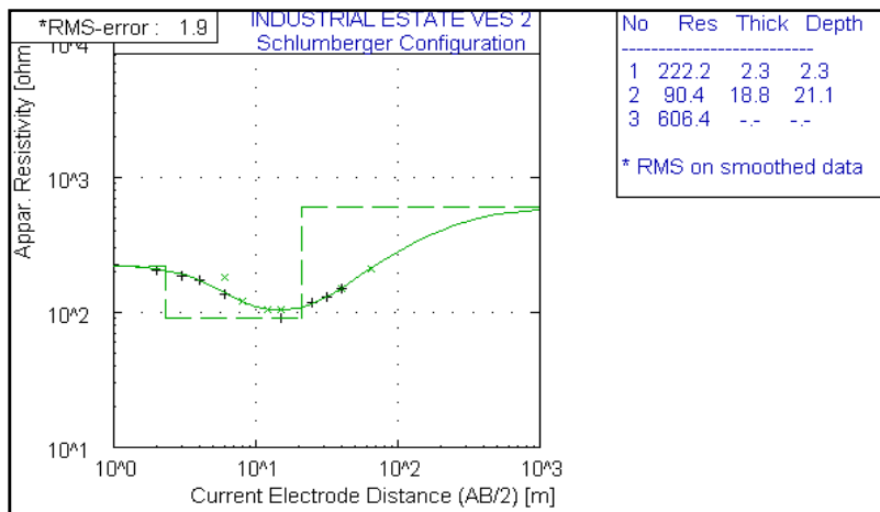
(b) The modeled curve for VES 2
