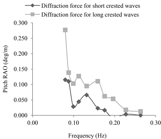
Fig. 8: Pitch RAO for wave directions comparison
