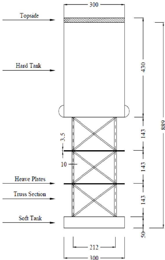
Fig. 2: Truss spar model configurations (in mm)
