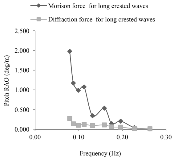
Fig. 5: Pitch RAO for wave force theories comparison
