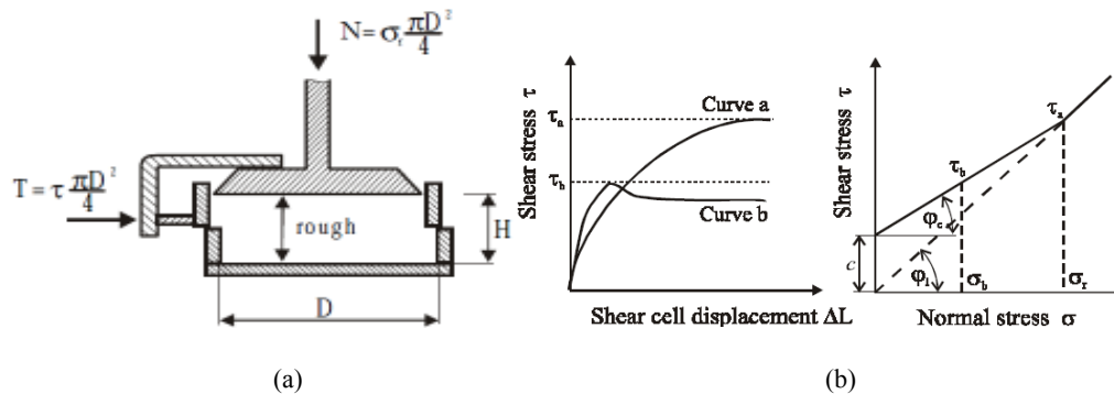
Fig. 1: Jenike shear tester and its relevant diagram: (a) Jenike shear tester, (b) relevant diagram of shear test
