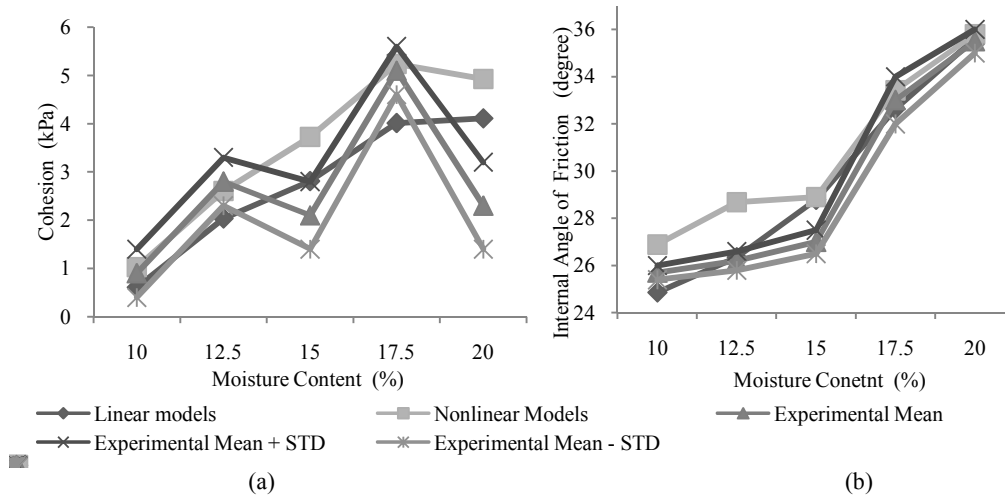
Fig. 4: Variation of strength properties of wheat grains with moisture content, Experimental and simulation results, (a) cohesion variation with MC, (b) internal angle of friction variation with MC
