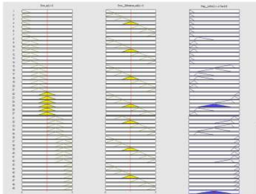
Fig. 2: Fuzzy control output representation of temperature control
