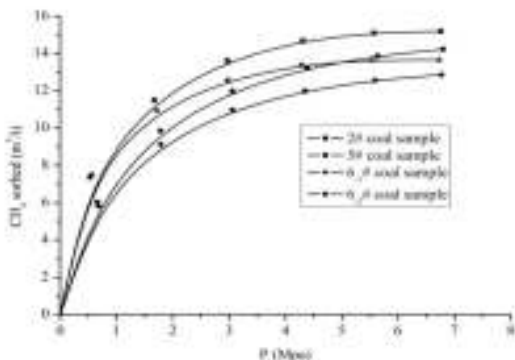
Fig. 3: The adsorption isothermal curve of coal samples of No.2 hole in Huale exploration region
