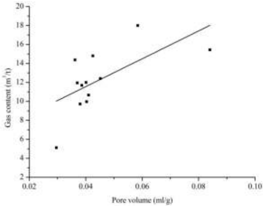
Fig. 7: Graph of pore volume and content of gas
