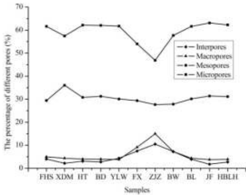
Fig. 6: The percentage of different pores sizes of different coal samples
