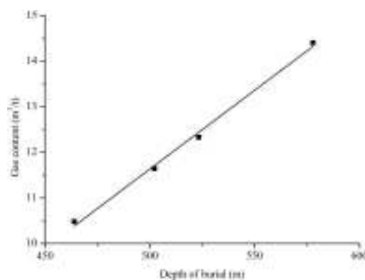
Fig. 5: Relational graph of depth of burial and gas content in Huale exploration region
