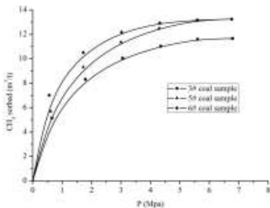
Fig. 2: The adsorption isothermal curve of coal samples of No.1 hole in Huale exploration region
