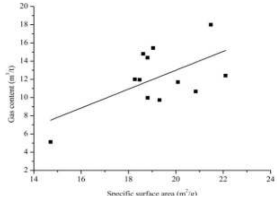
Fig. 9: Graph of specific surface area and content of gas
