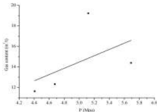
Fig. 4: Relational graph of reservoir pressure and gas content in Huale exploration region
