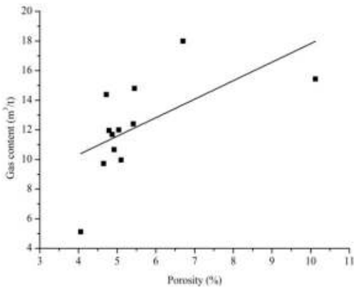
Fig. 8: Graph of porosity and content of gas
