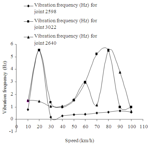
Fig. 14: The values of vibration frequency for joint 2598, joint 3022 and joint 2640
