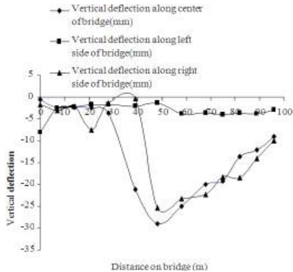
Fig. 11: The vertical deflection due to load combination II; (a) vertical deflection curve, (b) distribution of vertical deflection on longitudinal bridge model
