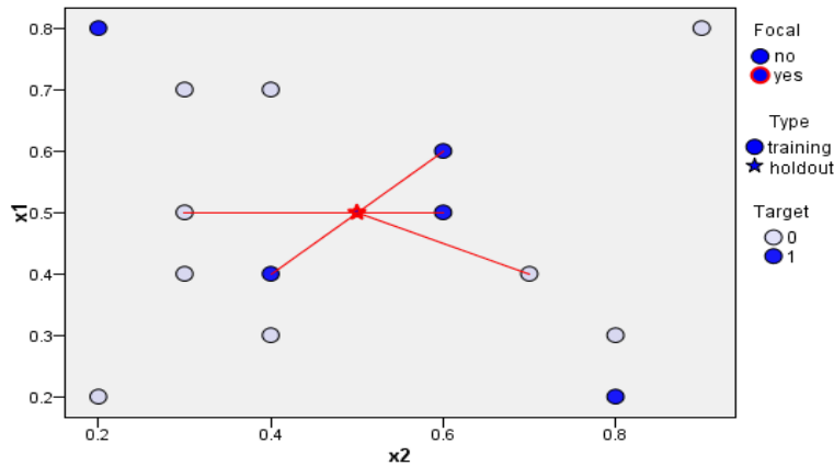
Fig. 1: Shown distance between the holdout point (star) and the training point (blue/white)
