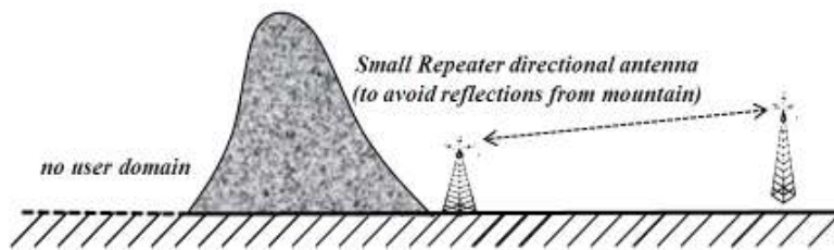
Fig. 13: Repeater placement of users centralized on one side
