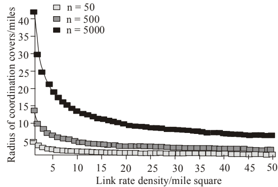
Fig. 17: Relationship between radius and density
