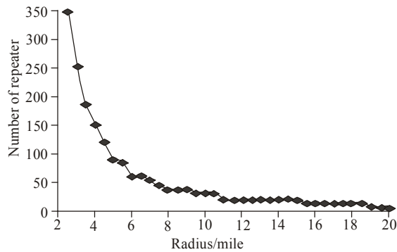
Fig. 3: Relationship between coverage radius and minimal number
