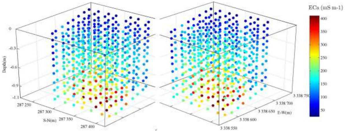
Fig. 1: Conductivities at 56 positions predicted from EM38 linear model; the two sides of the Figure form a stereogram which should be viewed with a pocket-stereoscope
