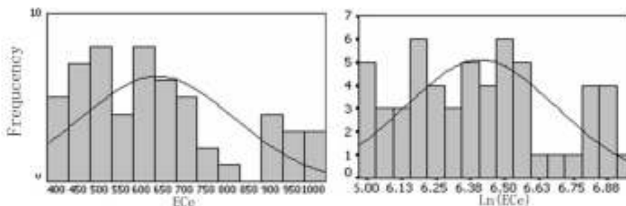
Fig. 2: Histograms on original scales (left) and on transforming to natural logarithms (right)depth, coefficients of variations became more and more small.
