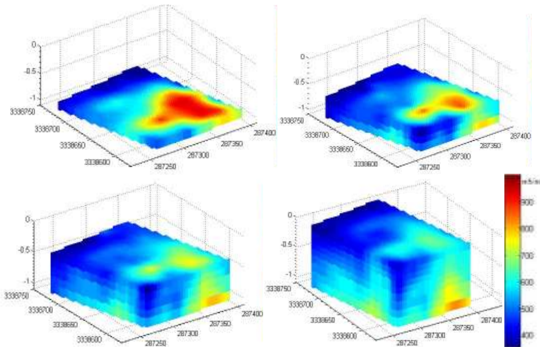
Fig. 3: Three dimensional space distribution of soil ECe by disjunctive kriging
