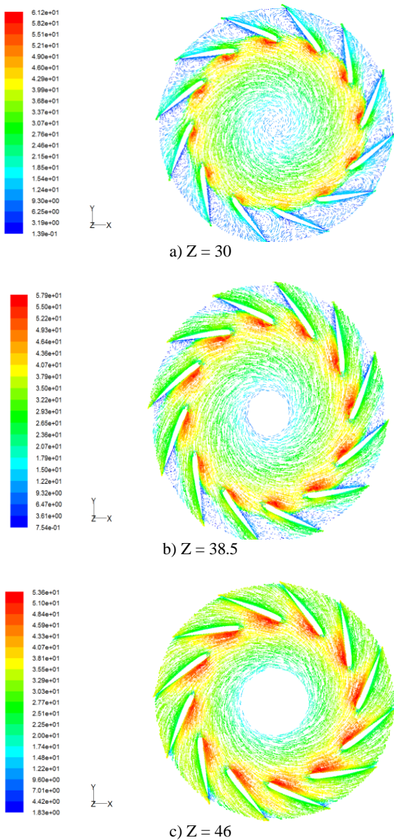
Fig. 9: Vectors of relative speed at different axial cross sections when k_1=0.89 (The 170th rotational period)
