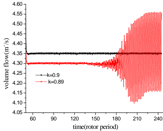
Fig. 4: Flowrate variations with time on two valve opening
