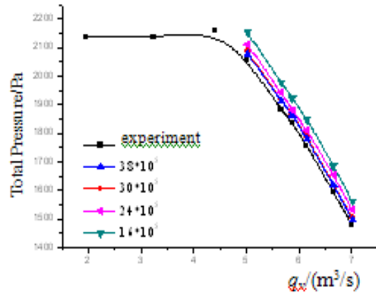
Fig. 3: Relation of full pressure and flowrate
