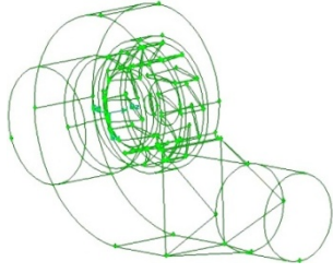
Fig. 1: Geometric model of centrifugal fan
