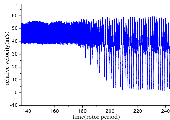
Fig. 6: Relative speed variation with time
