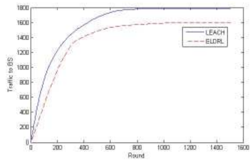
Fig. 12: Snapshot of the network traffic (field 300\text{ m}^2 )
