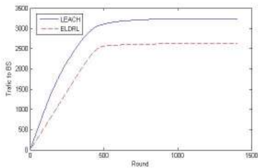
Fig. 11: Snapshot of the network traffic (field 200\text{ m}^2 )
