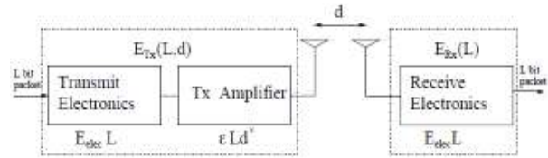
Fig. 7: Radio energy dissipation model
