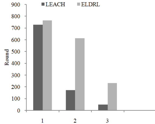
Fig. 8: Results for a network with different field of sizes for ELDRL when the first node dies
