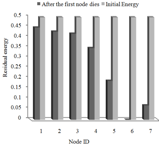
Fig. 3: Energy dissipation
