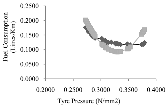
Fig. 4: Model values of Vehicle No.1 compared to the measured value
