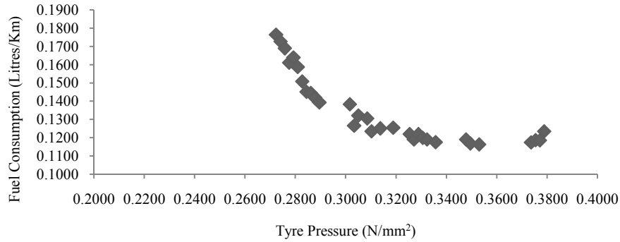
Fig. 2: A scatter diagram for Vehicle No.1 showing fuel consumption verses tyre pressure
