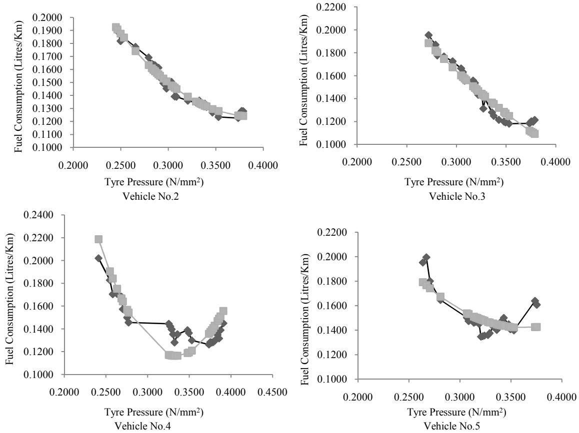
Fig. 5: Model values of Vehicles No. 2, 3, 4, and 5 compared to the measured values respectively
