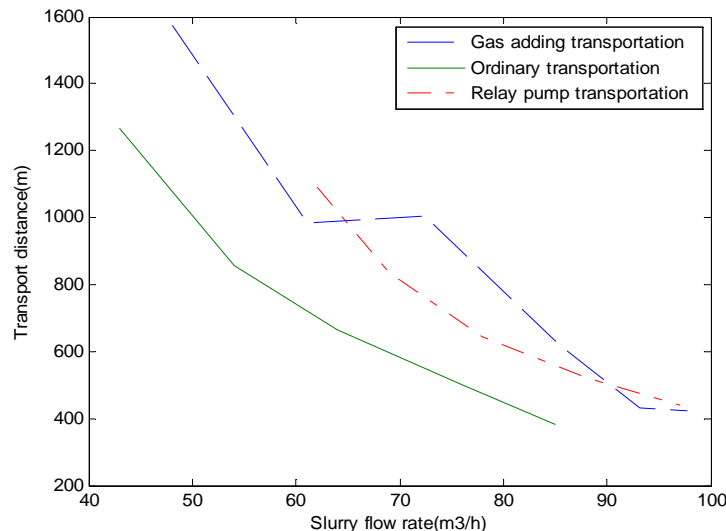
Fig. 7: Transport distance in different transport means
