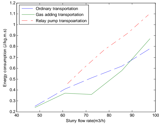
Fig. 8: Unit energy consumption in different transport means
