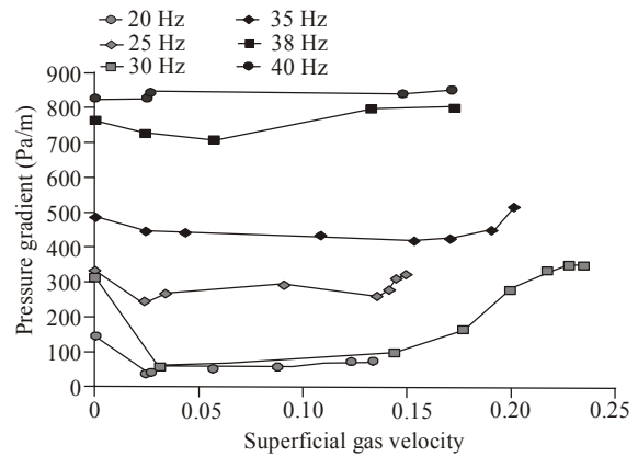
Fig. 4: Relation between pressure gradient and superficial gas velocity under different frequencies of main pump
