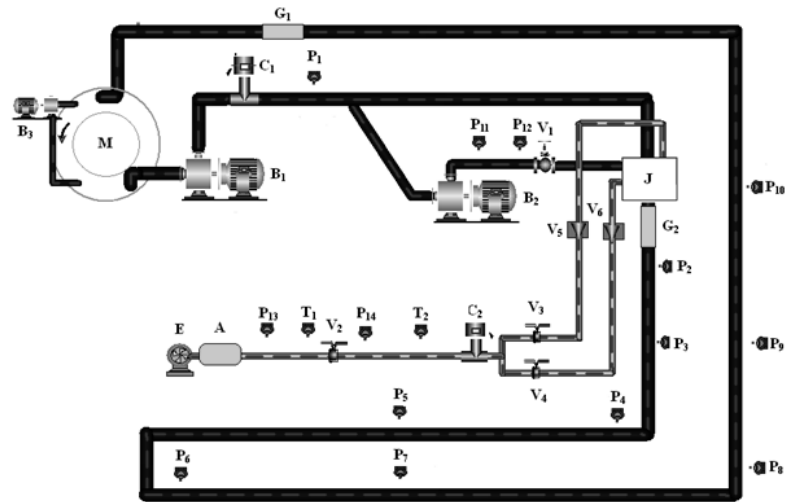
Fig. 1: Hydraulic circuit of the pipeline apparatus; A-air tank; B1-primary pump; B2-jet pump; B3-agitator pump; C1-electromagnetic flow meter; C2-air flow meter; E-compressor; G1,G2-transparent glass pipes; J-air injector; M-slurry pool; P1 to P14-pressure transducers; T1,T2-temperature sensors; V1-ball valve; V2-pressure relief valve; V3,V4-valves; V5,V6-Single-phase Valves
