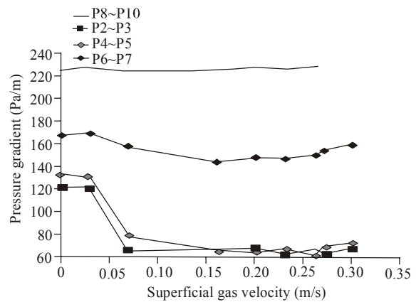
Fig. 6: Relation between pressure gradient and superficial gas velocity in different spots of pipe
