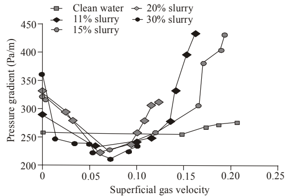
Fig. 5: Relation between pressure gradient and superficial gas velocity under different slurry concentrations
