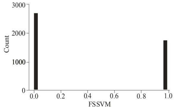
Fig. 3: Dataset analysis
