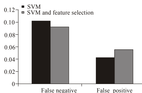
Fig. 7: False positive and false negative comparisons between SVM and hybrid SVM
