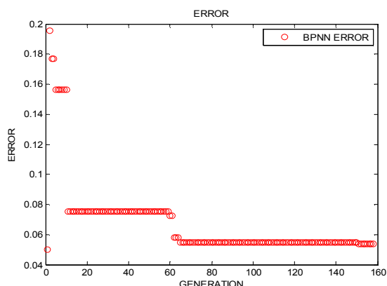
Fig. 7: GA-ELNN error
