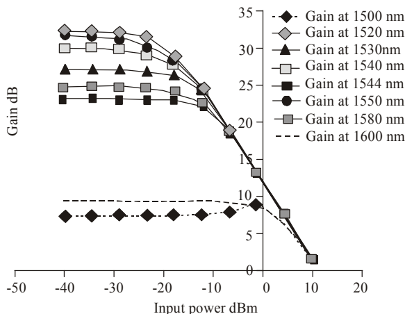
Fig. 6: SOA gain at different \lambda (nm)
