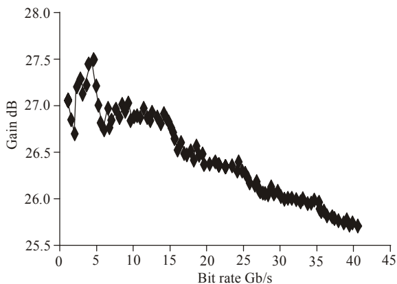
Fig. 7: SOA gain at -25 dBm
