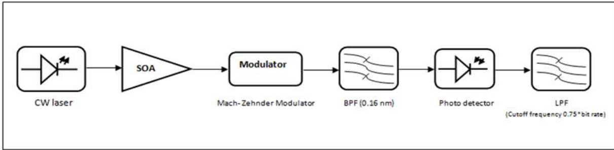
Fig. 1: Simulation set-up
