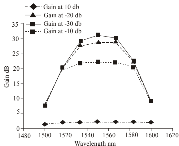
Fig. 5: SOA gain for different input power
