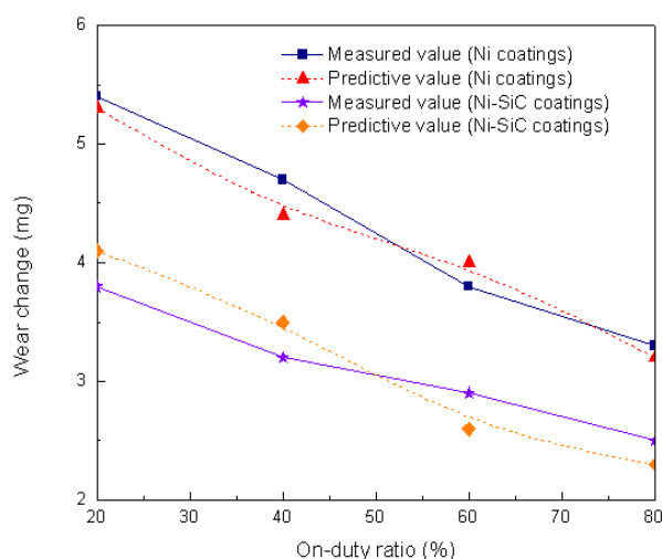
Fig. 5: Effect of on-duty ratio on wear loss of coatings
