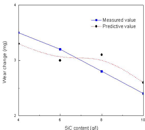
Fig. 3: Effect of SiC content on wear loss of coatings
