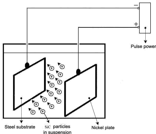
Fig. 2: Schematic diagram of the electrodeposition cell
