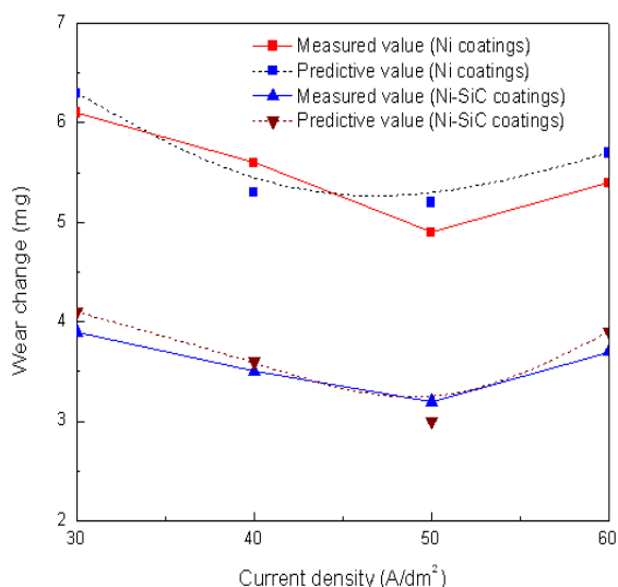
Fig. 4: Effect of current density on wear loss of coatings
