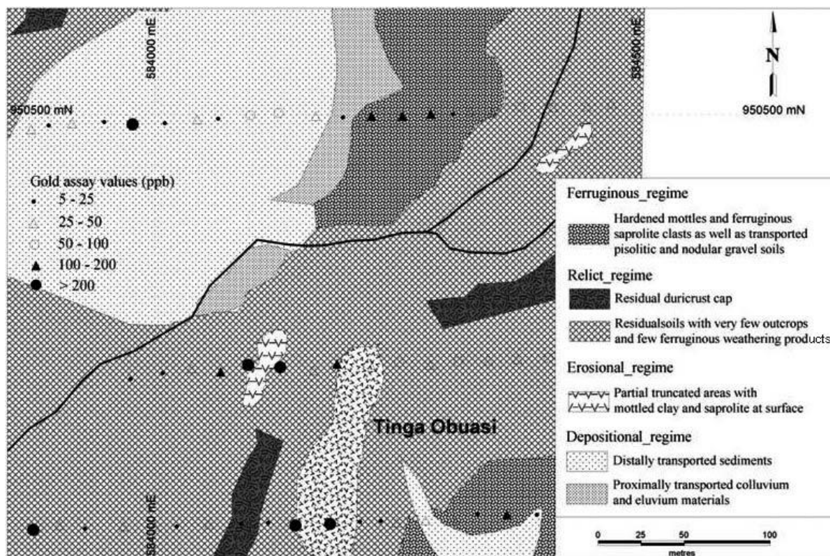
Fig. 3: Typical regolith map in northern Ghana (Arhin and Nude, 2009)
