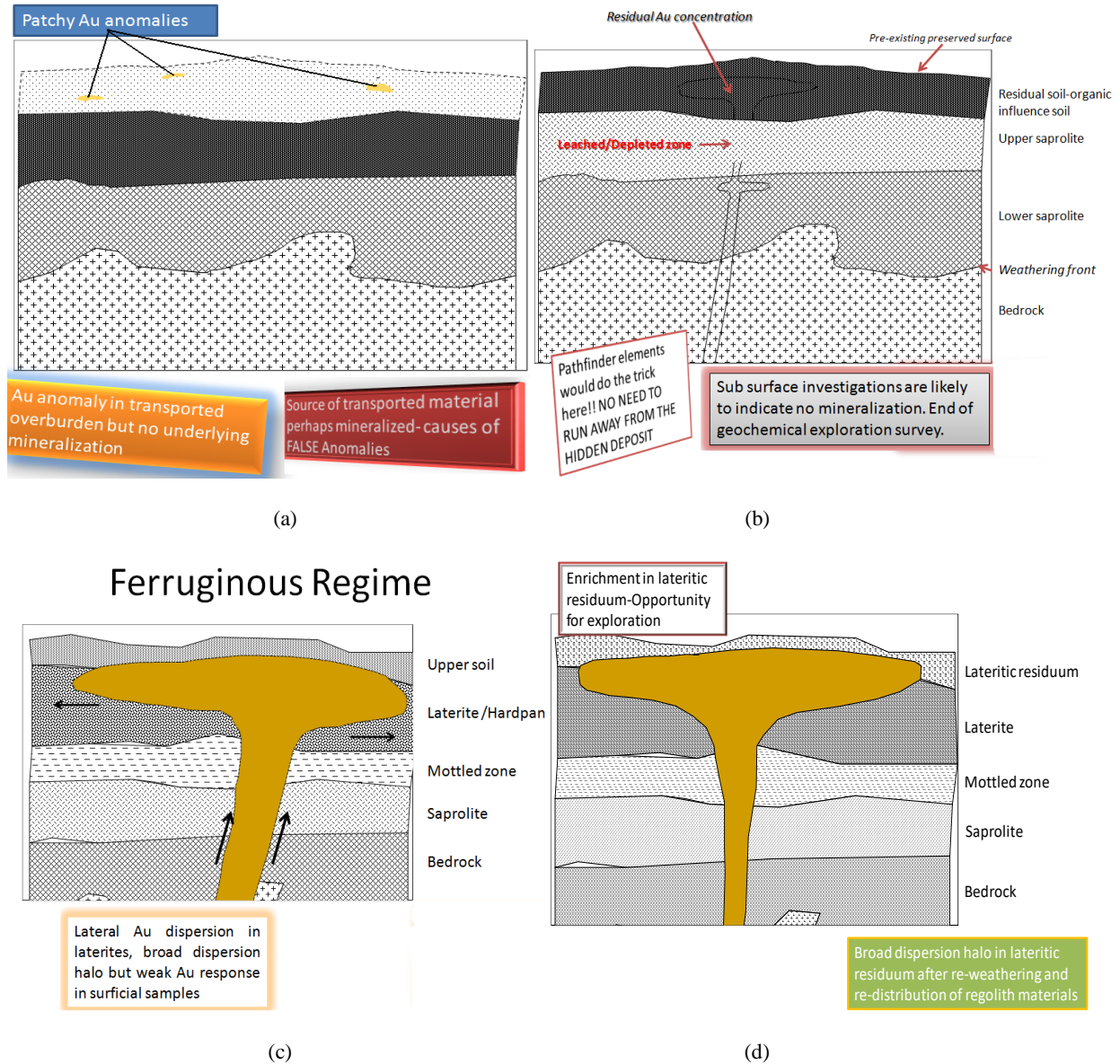
Fig. 2: Patchy and false anomalies resulting dispositional overburden or thick ferruginous enrichment
