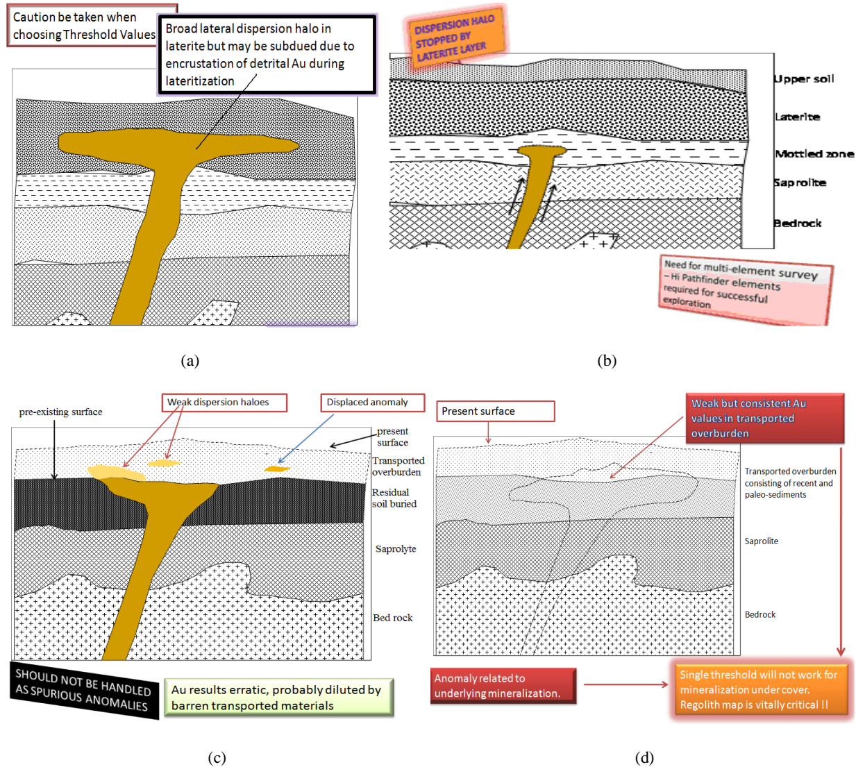
Fig. 5: Some exploration issues from landform modifications and variable
