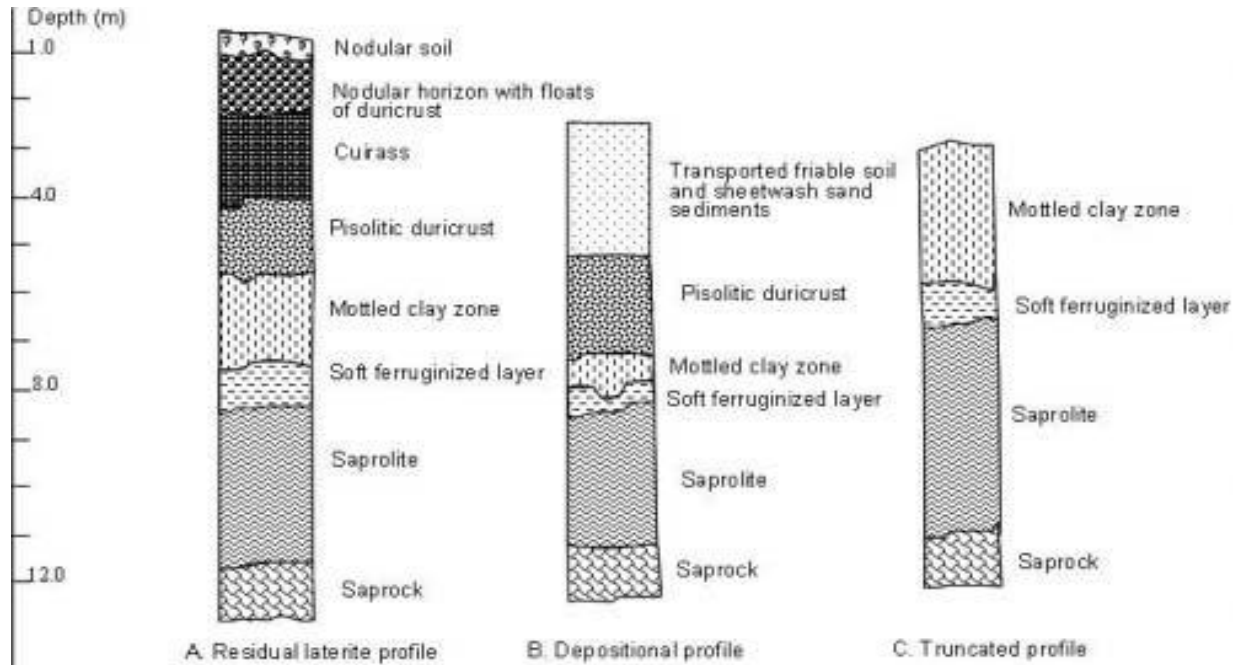
Fig. 4: Typical regolith stratigraphy in study area (Arhin and Nude, 2009)
