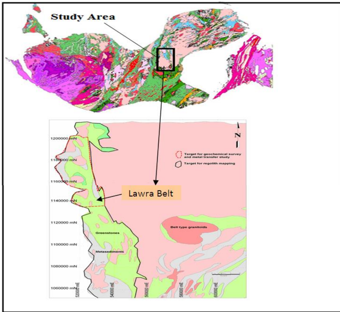
Fig. 1: Geology and location of study area (modified after Arhin and Nude (2009))
