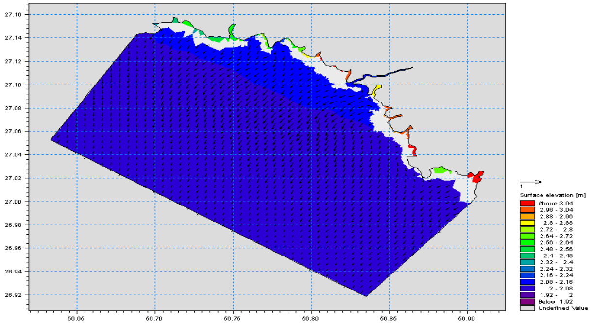
Fig. 13: Example of a two-dimensional model of tidal currents in the ebb range plan
