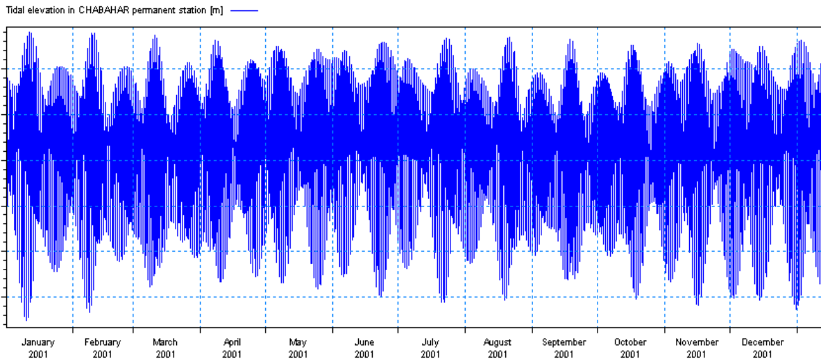
Fig. 6: Time series of tidal elevation martyr Beheshti port of Chabahar (regional model boundary information)
