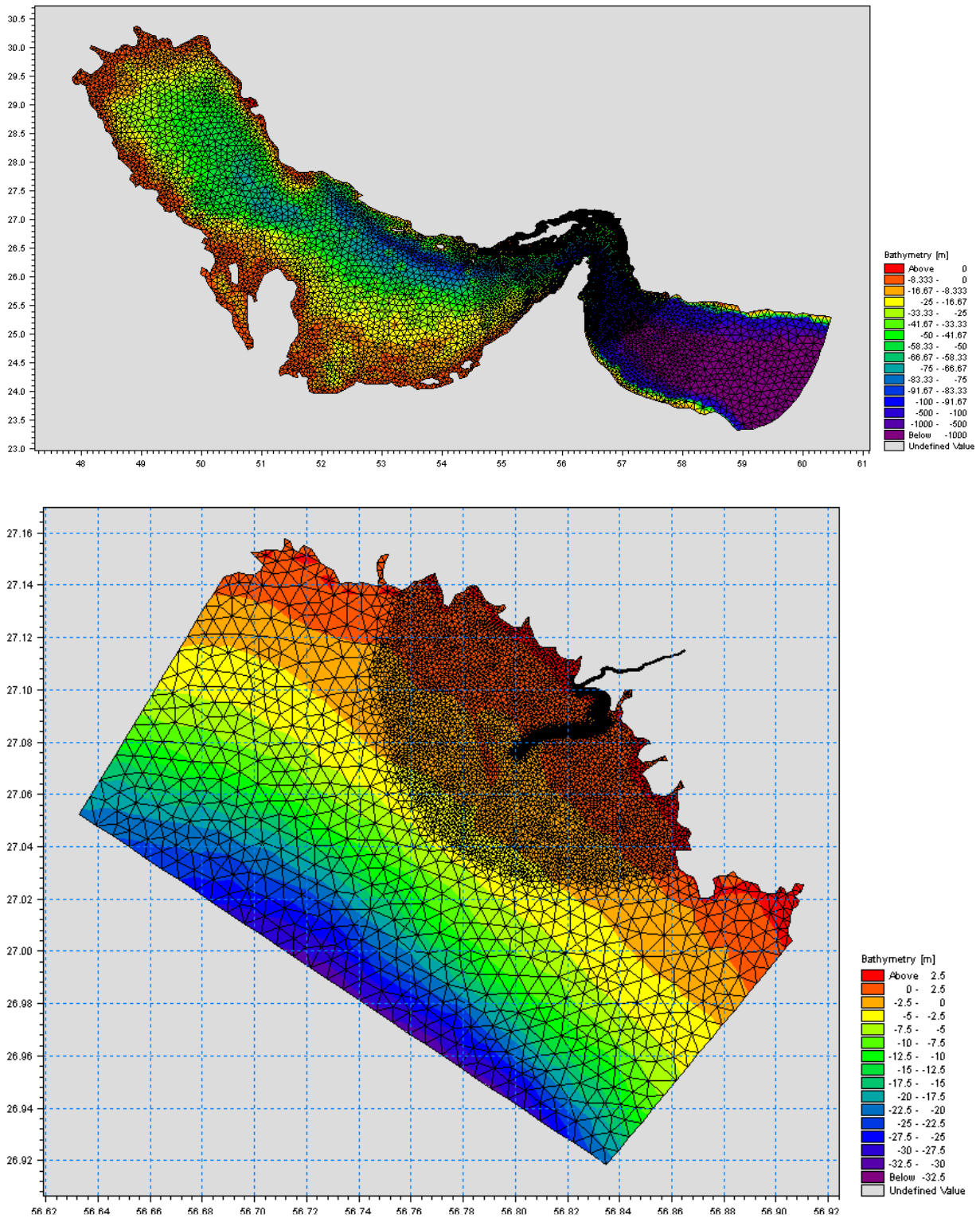
Fig. 4: Regional and local mesh models
