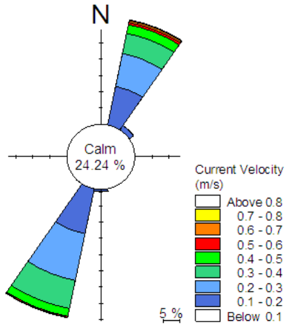
Fig.19: Flow flower creek trailhead (T1)
