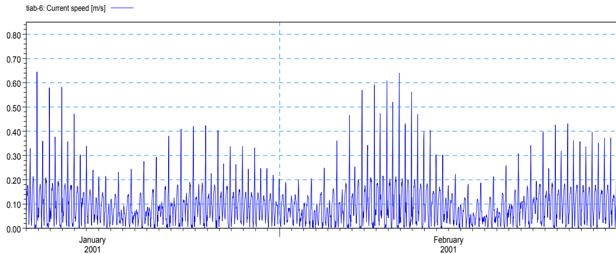
Fig. 18: Changes in the flow rate of the feed point at a depth of-2 m
