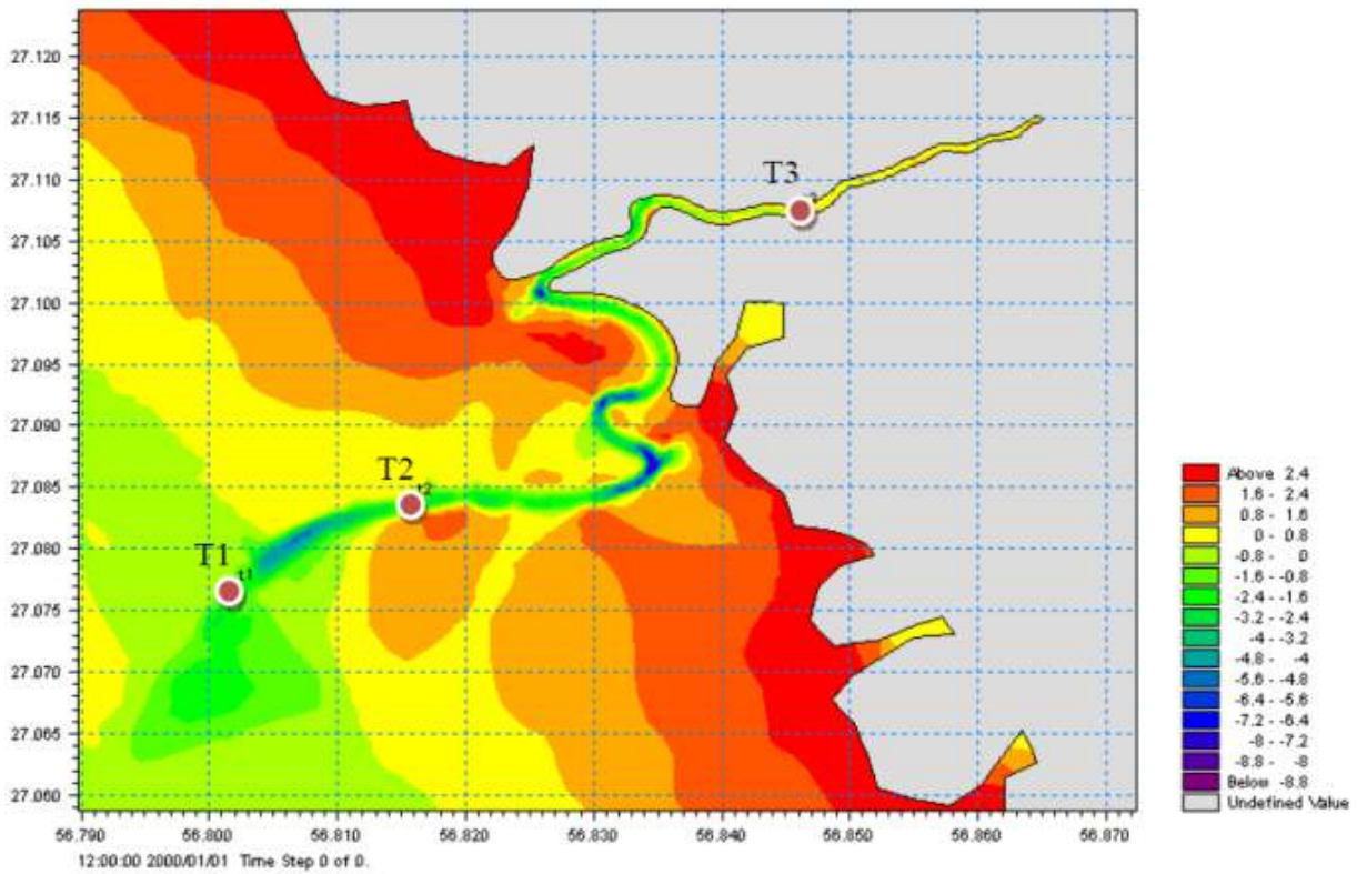
Fig. 10: Location of the estuary to extract modeling results
