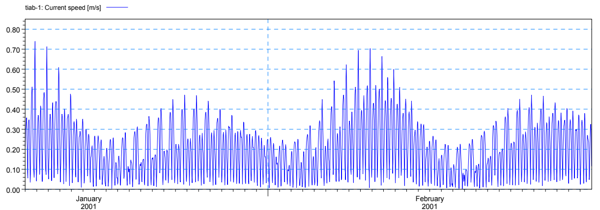
Fig. 15: Changes in the estuary of the river flow rate at the beginning (T1)
