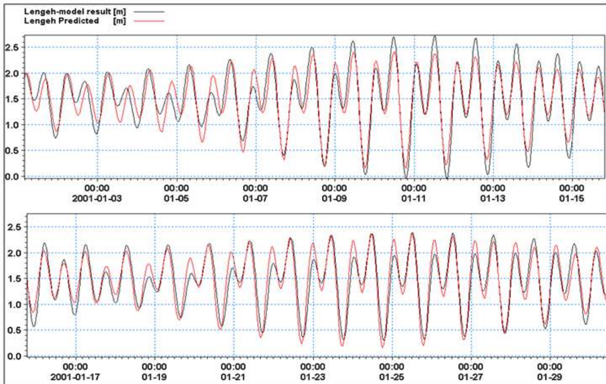
Fig. 8: Comparison of model results and predictions made for the water level station LENGHEH
