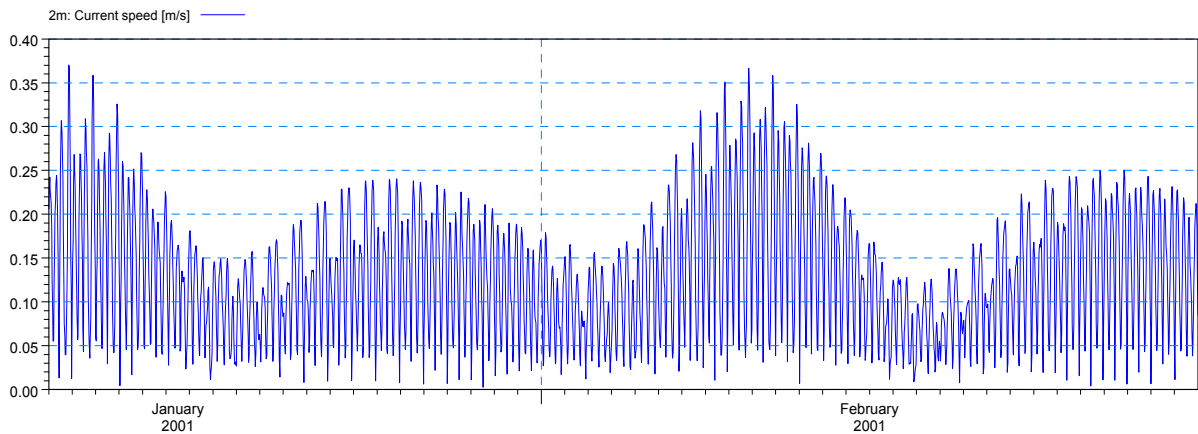
Fig. 17: Flow velocity changes in internal point along the estuary near the mouth (T3)
