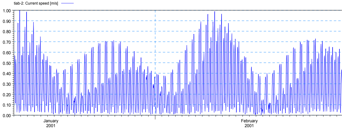
Fig.16: Flow velocity changes in internal point along the estuary near the mouth (T2)
