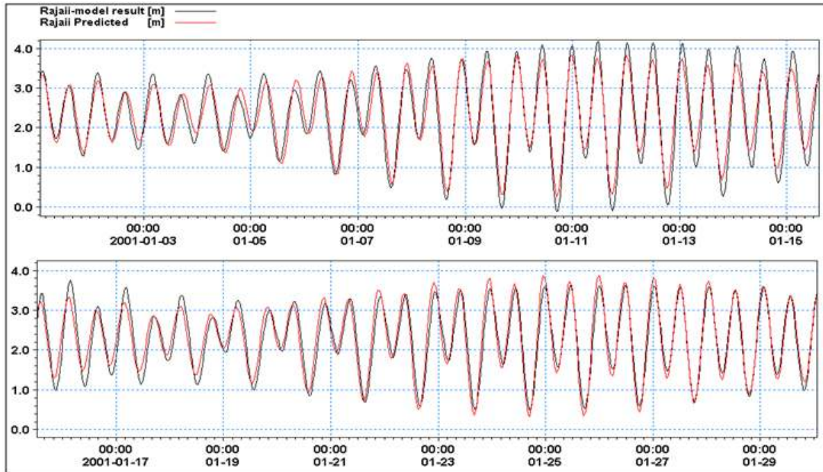
Fig. 9: Comparison of model results and predictions made for the water level station martyr Rajai Port
