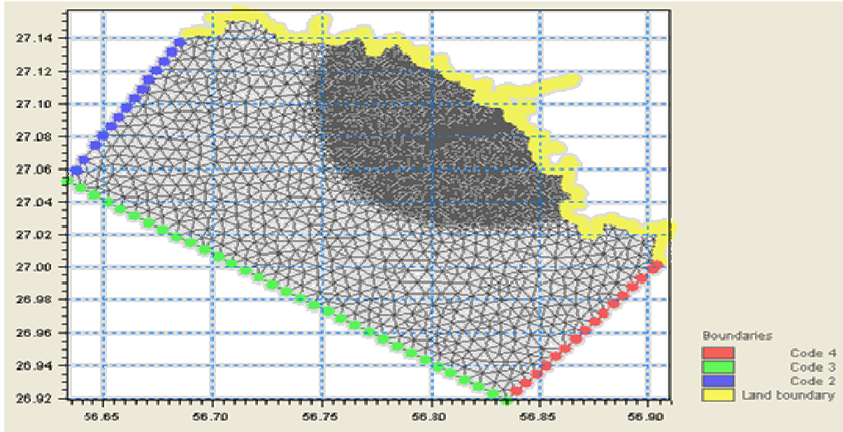
Fig. 7: Location and type of boundary conditions selected for local modeling
