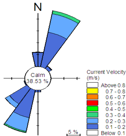
Fig. 21: Flowers in the interior point along the estuary (T3)
