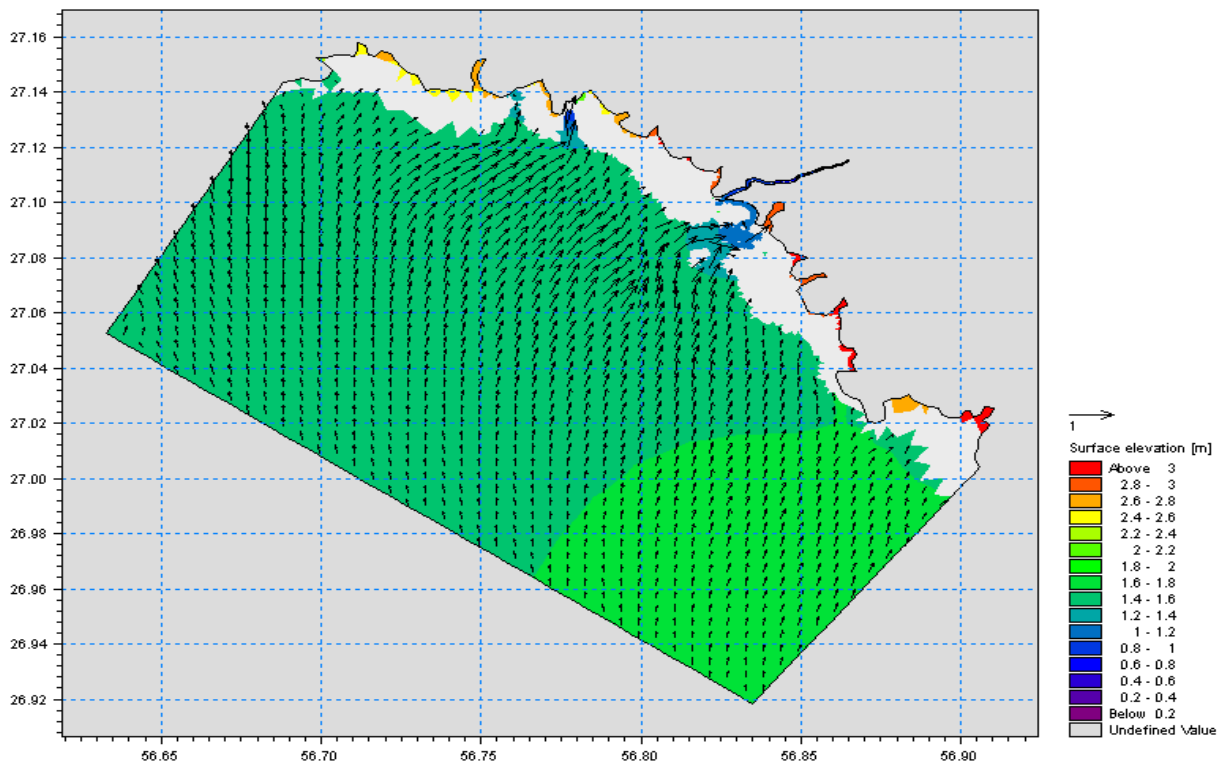
Fig. 12: An example of a two-dimensional model of tidal currents in design area in flood state
