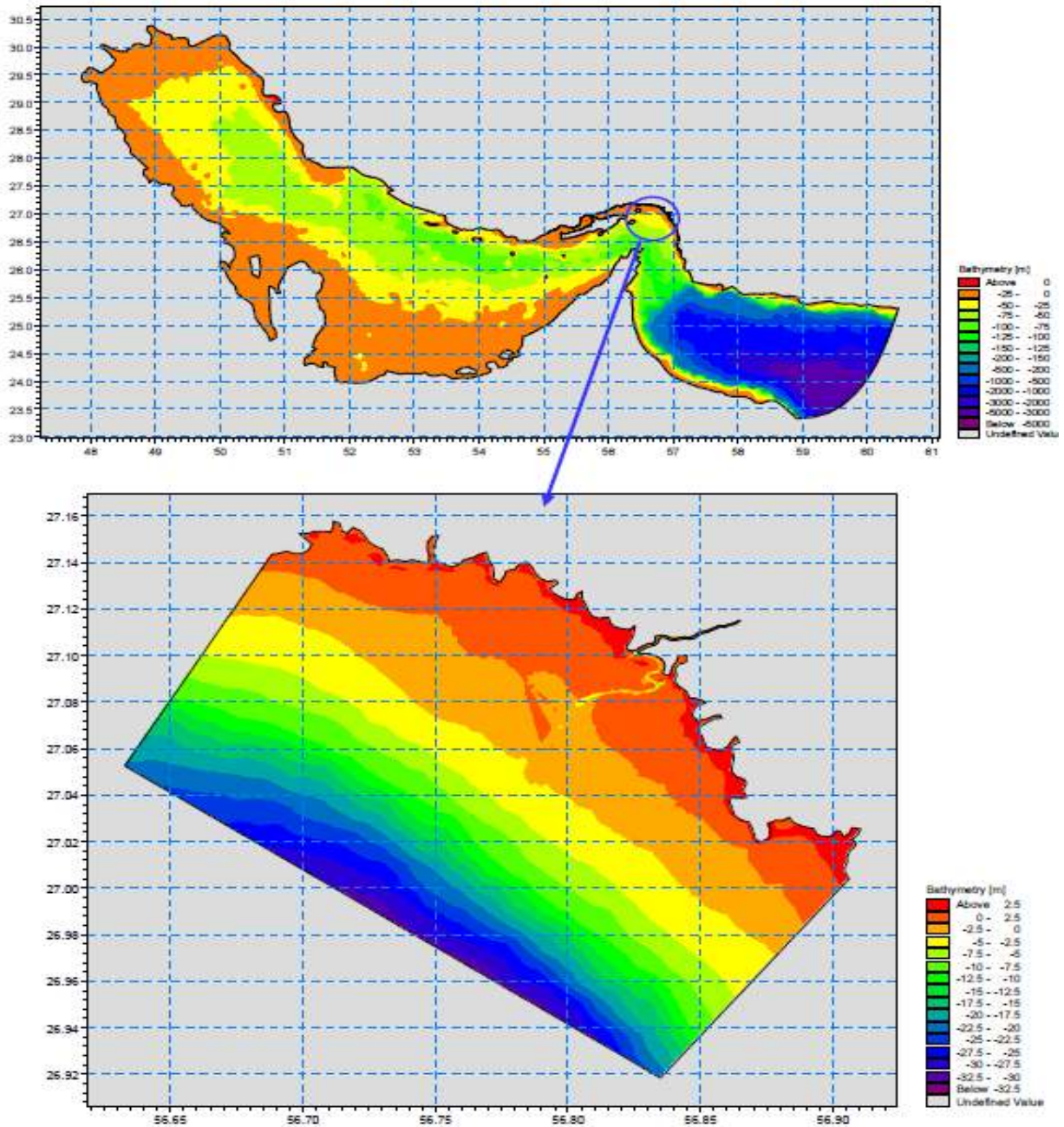
Fig. 3: Model of regional and local
