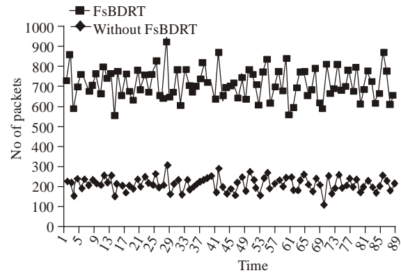
Fig. 7: Overall performance analysis of (Fs BDRT) 5 packet/sec
