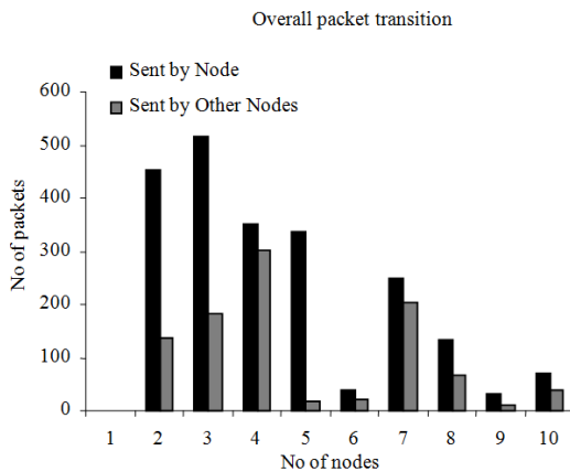
Fig. 5: FsBDRT performance on 50 % of congestion
