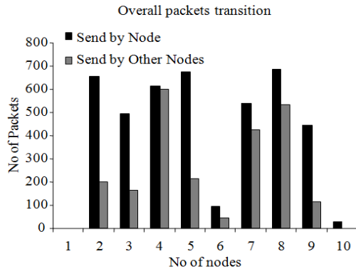
Fig. 9: Fs BDRT performance on 50 % of congestion (10 packets/sec)
