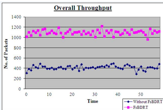
Fig. 11: Overall performance analysis of (FsBDRT) 10 packet/sec
